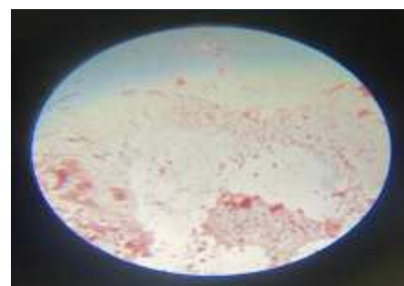
Fig.5 (Endospore staining)
