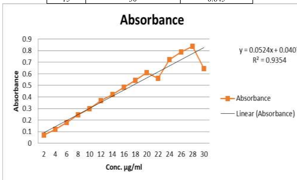
Fig. No. 1.8 –Calibration curve of Modified folic acid in pH 6.8 at 282 nm
