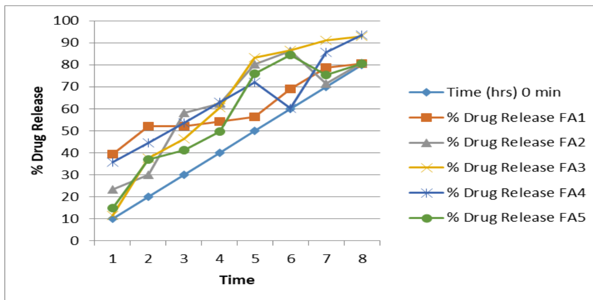
Fig. No.1.12 – Comparison of % drug release through tablet from goat intestinal mucosa
