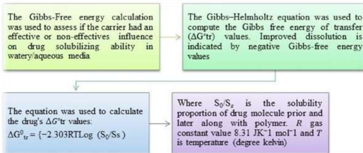
Figure 1.6 Gibbs-Free Energy Calculation [70]
