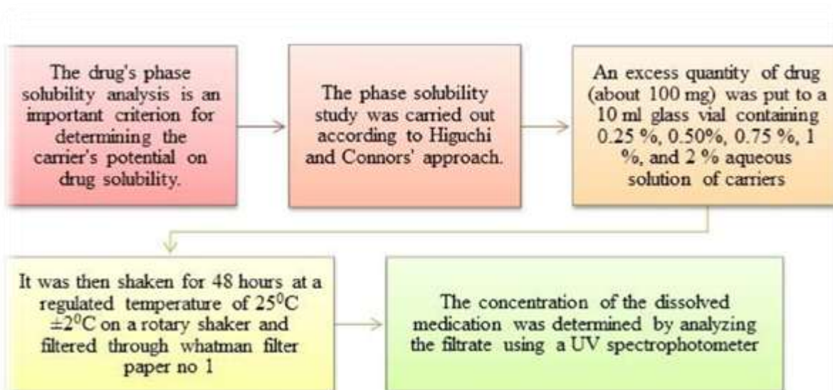
Figure 1.5 Phase Solubility Study of Drug [69]
