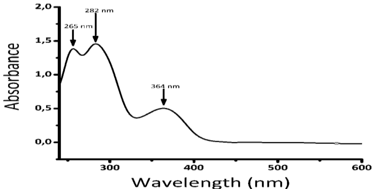
Fig No. 1.7 –Spectrum of Modified Folic acid in pH 6.8 Solution
