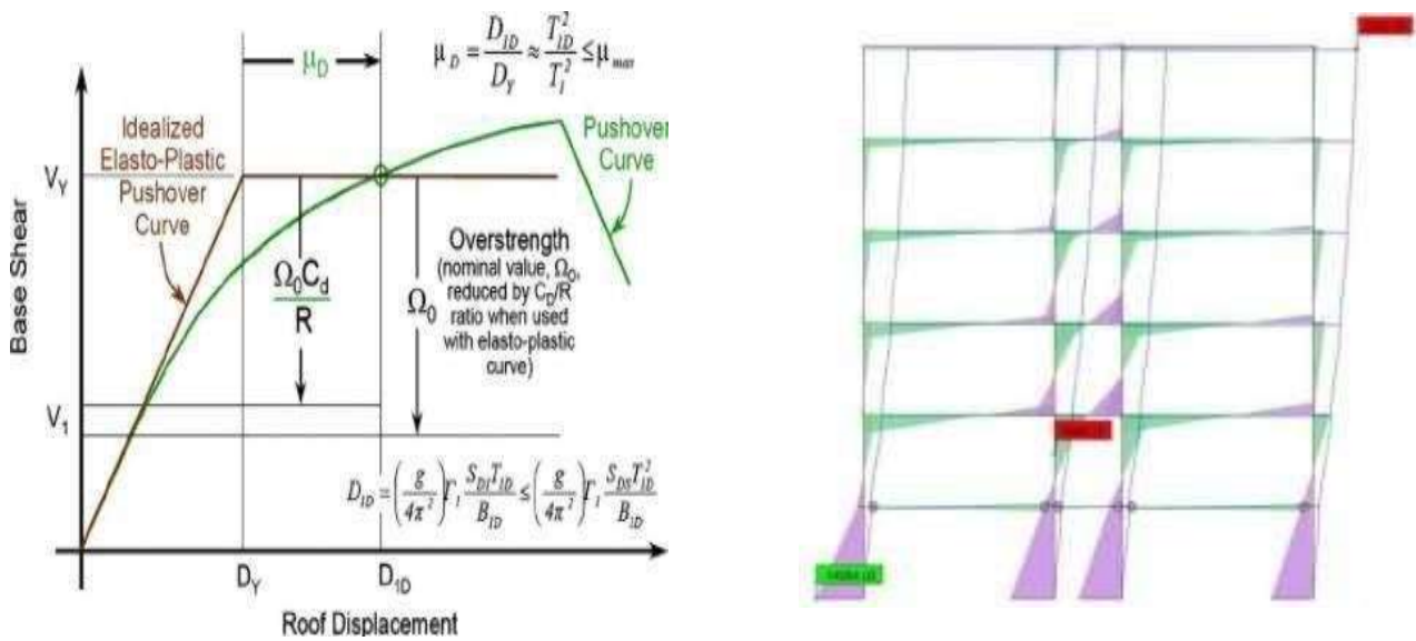
Fig 1: Pushover Analysis
