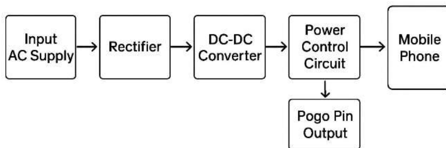
Figure 1: Block Diagram of Universal Mobile Charger
