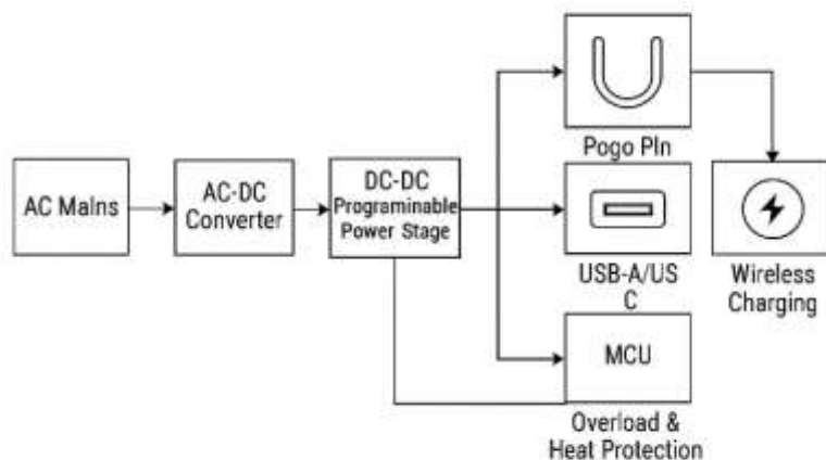
Figure 2: Smart Charging System Architecture
