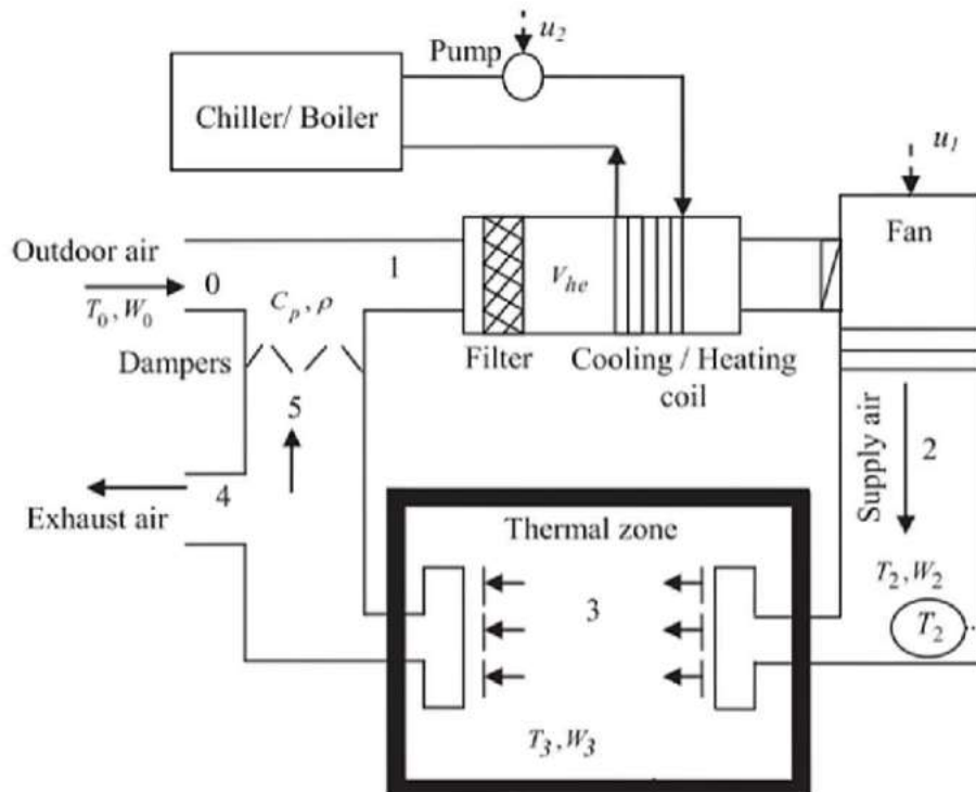
Figure 1: Block diagram of a simple HVAC system (M. Gomez)
