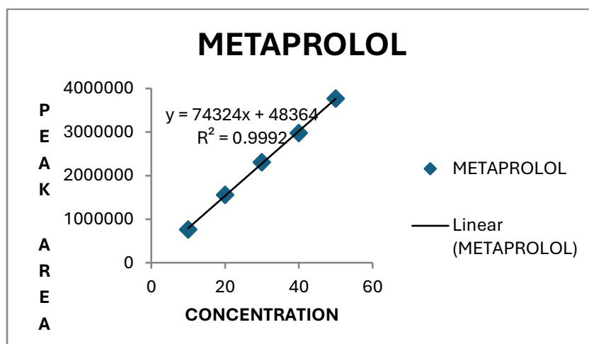
Fig 4: Calibration curve for linearity of Metoprolol succinate with peak area
