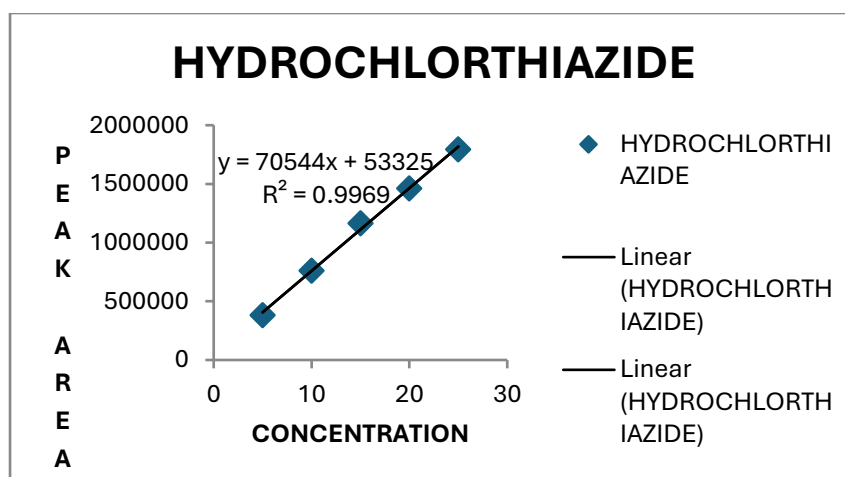
Fig 5: Calibration curve for linearity of Hydrochlorothiazide with peak area
