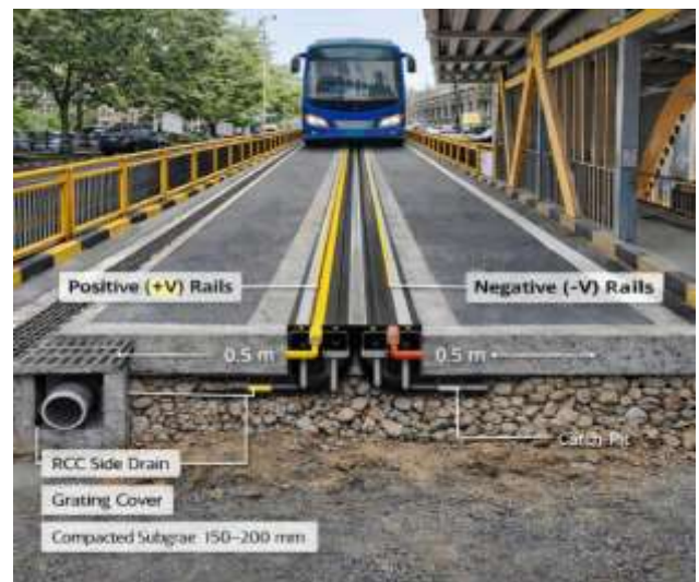
Fig. 1.1 SECTION OF ROAD
