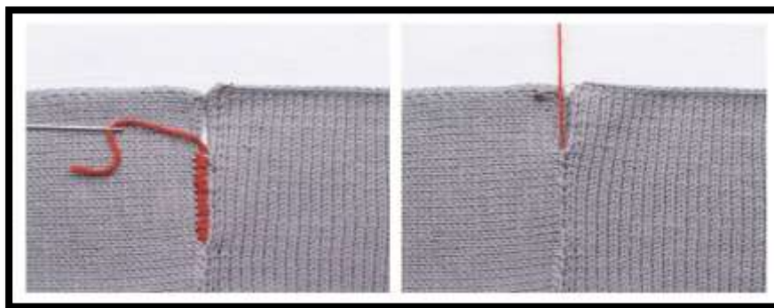
(Seaming)
